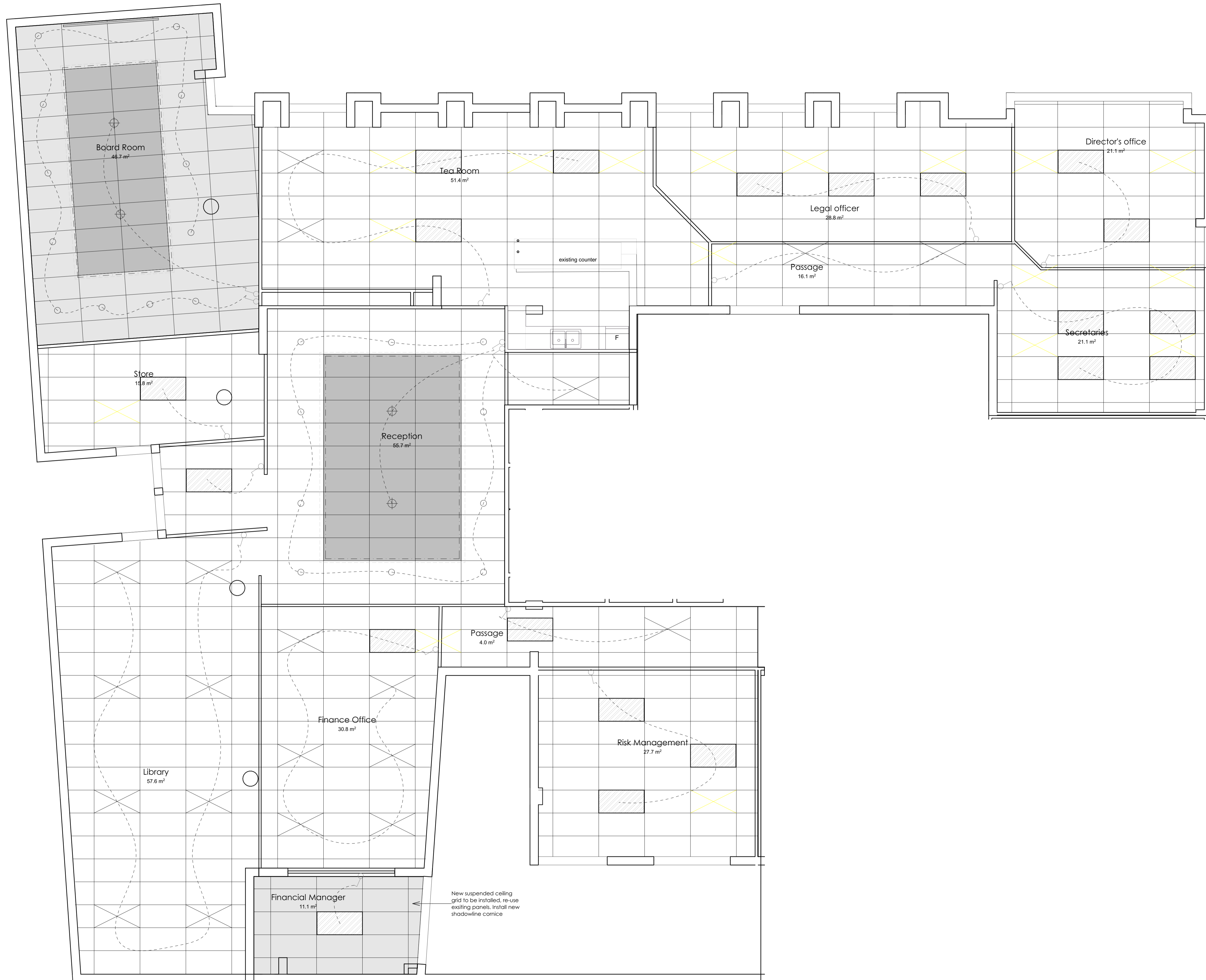
Ceiling & Lighting Plan Scale 1:50
